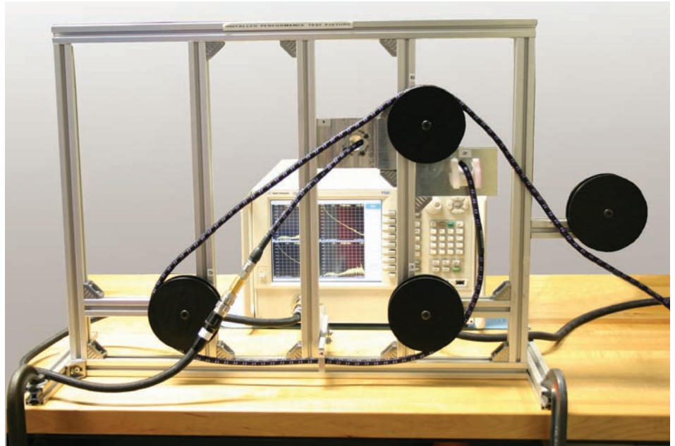
Figure 1: Installation Simulator
